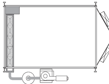
Simple Hopper, Excavated or Above Ground
