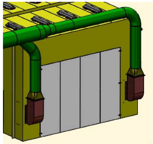
Outlet plenums of a 'Drive-Thru' type booth
